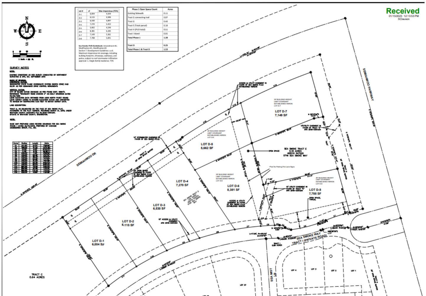
Figure 2- Proposed Plat Layout
